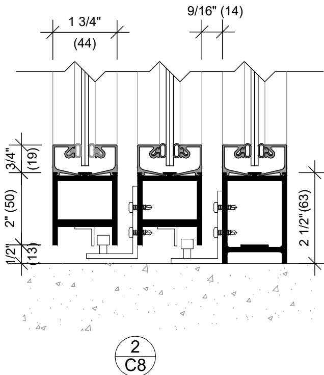
ALTERNATE RECESSED TRACK DETAILS
