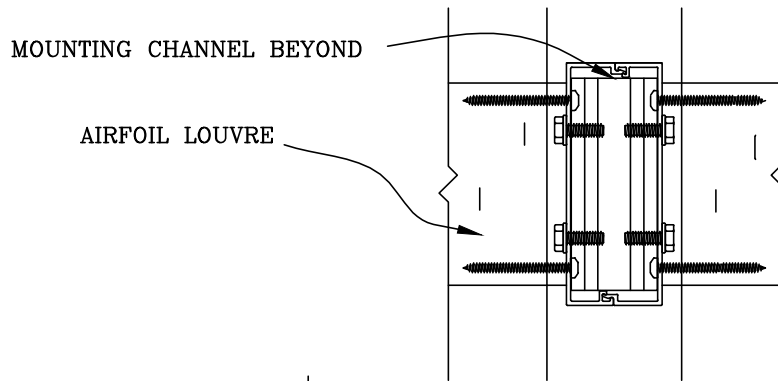
SUNSHADE OUTRIGGER DETAIL
