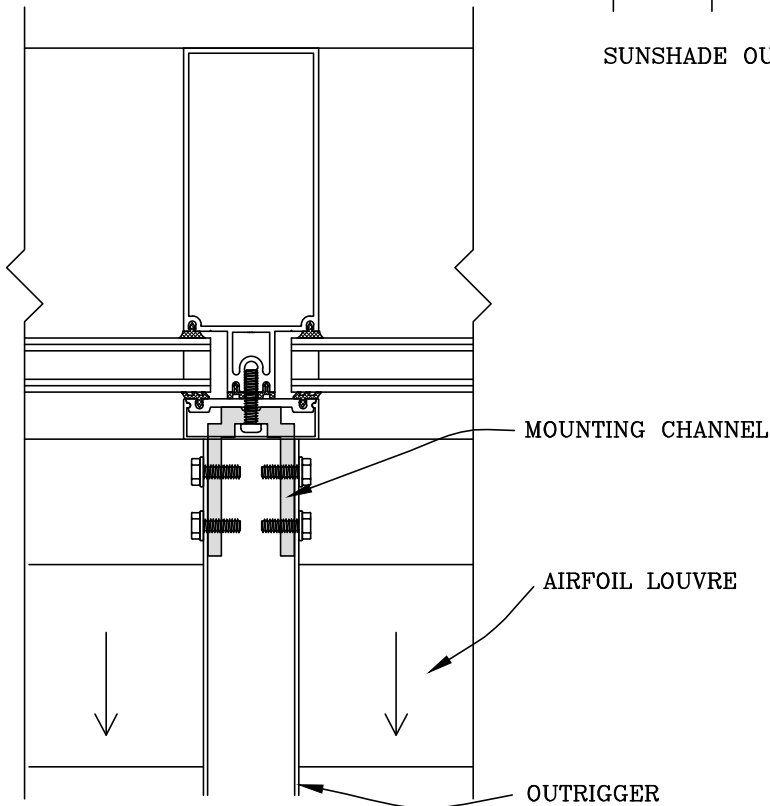
SUNSHADE MOUNTING DETAIL (SHOWN ON 2500 SERIES)
