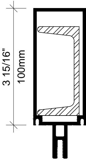
D4530 (C/W C3 X 4.1)
