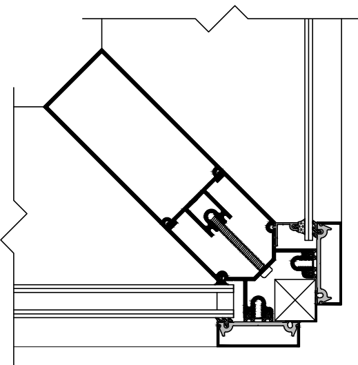
C2530 STANDARD CORNER
