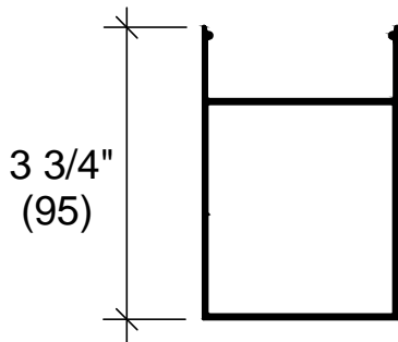
C2504 SNAP-ON CAP
