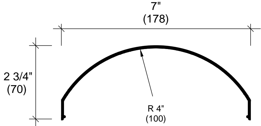
C2590 COLUMN CAP
