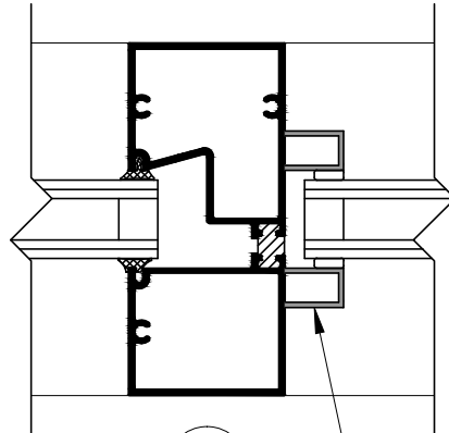
SCREW APPLIED VERTICAL STOPS ON TRANSOM
