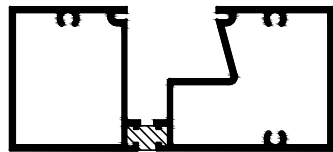
F2002 DOOR MULLION / HEAD
