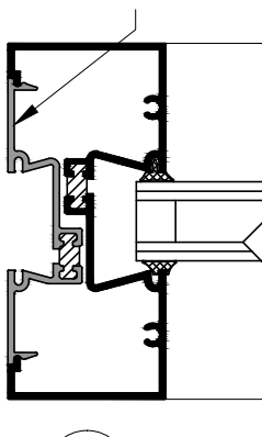
OPTIONAL FILLER FOR CLOSED BACK JAMB
